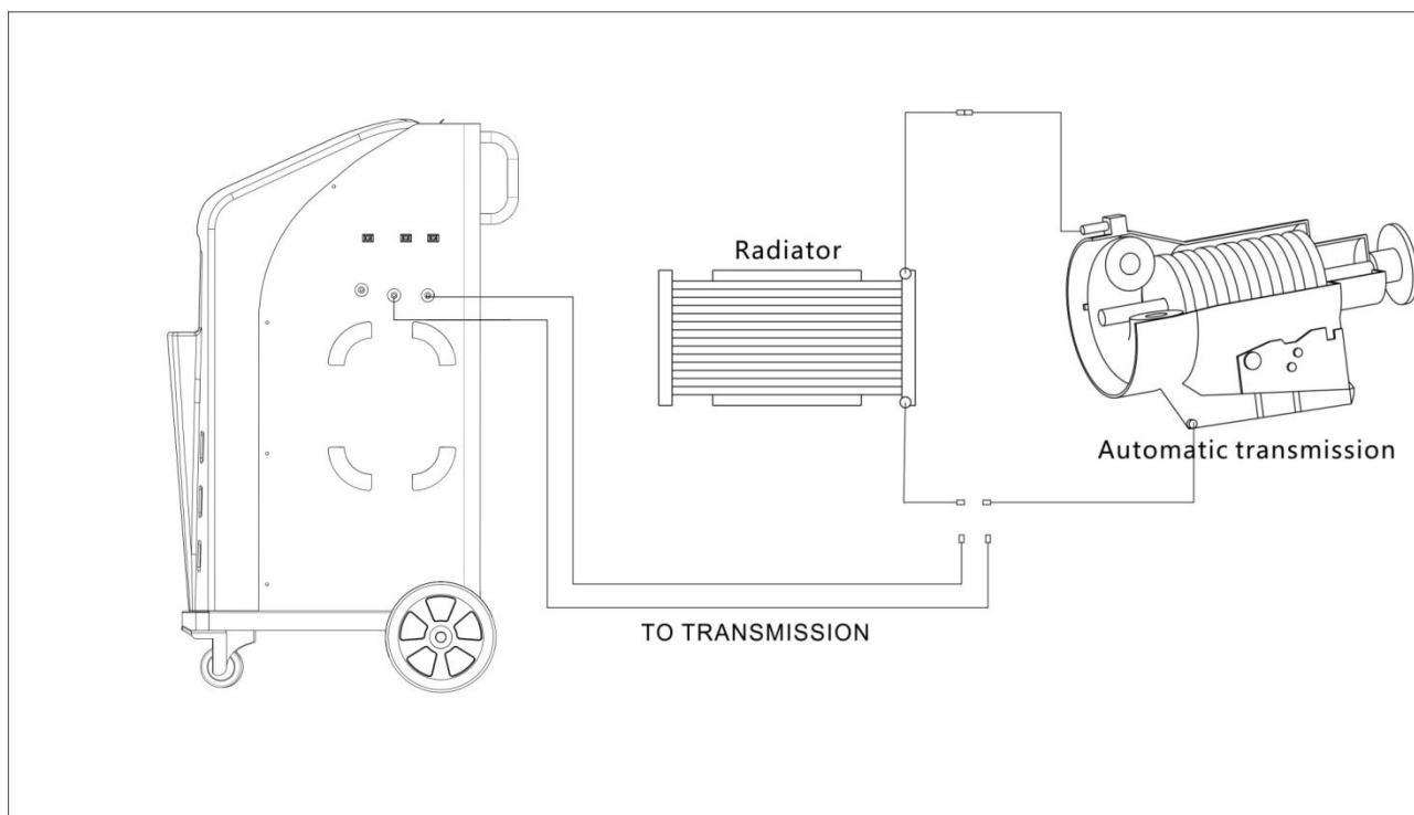
Pic. 3 Hose connection
